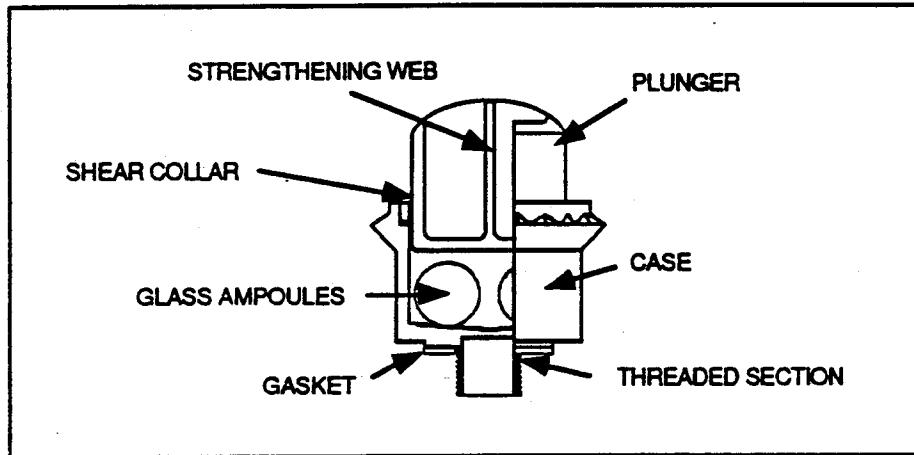
FIGURE 6 Anti-personnel
