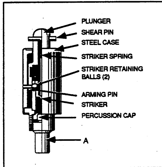
FIGURE 3 Model M/47-2
