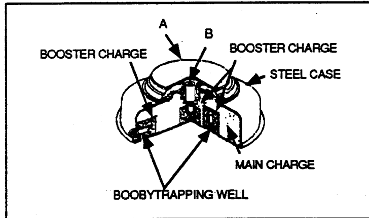
FIGURE 1 Model M/47-1
