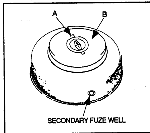
FIGURE 8 M15 Anti-Tank Mine
