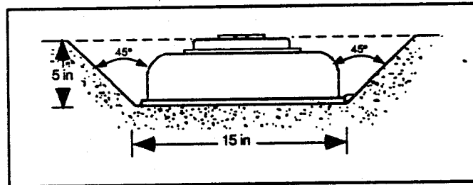
FIGURE 9 M15 Anti-Tank Mine
