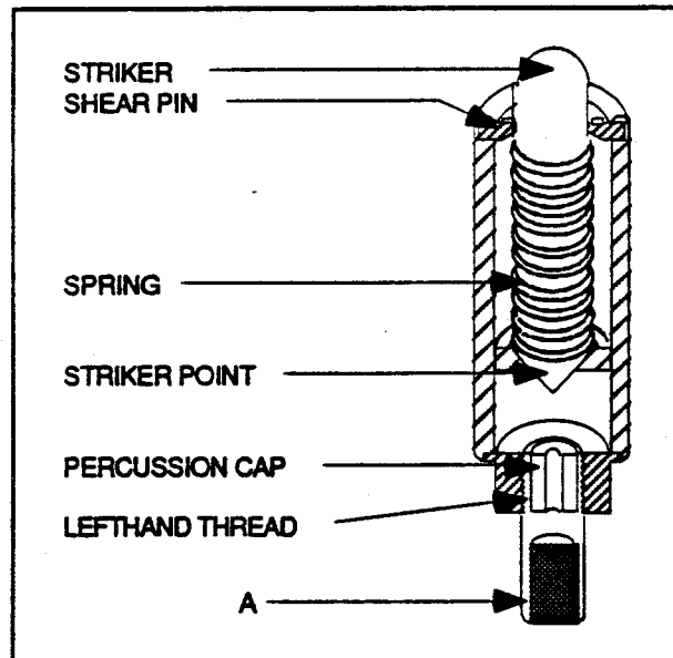
FIGURE 2 Model M/47-1
